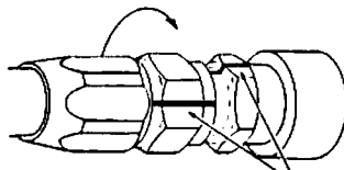
Misalignment of the mark shows the amount which the nut was tightened.
